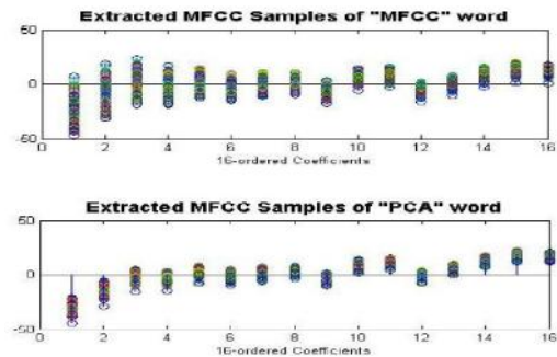
Figure 4. The 16-bit ordered MFCC extracted from voiced speech samples
