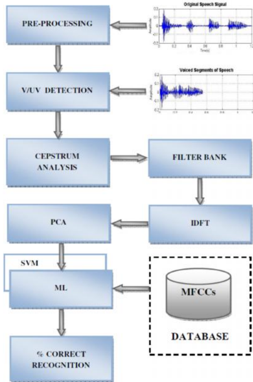
Figure 2. workflow for MFCC based speech classification.
