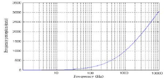
Figure 3. logarithmic plot of the mapping frequencies between 0 and 10 KHz.
